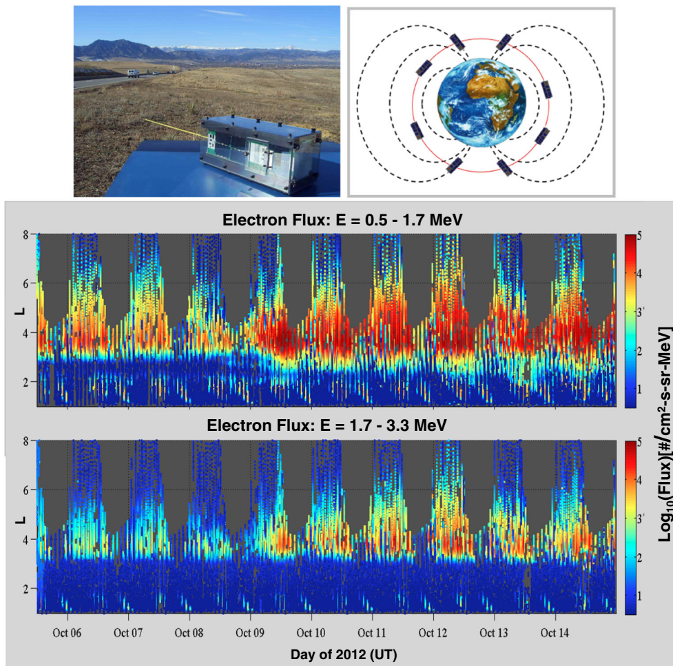
Figure 1. A picture of the CubeSat during testing (top left) and a schematic view of the CubeSat's orbit and orientation (top right)—the CubeSat has a passive magnetic attitude control system that will always try to align the long axis of the satellite with the local magnetic field. First 10 days measurement of the electron fluxes in different energy channels, color-coded in logarithm, and sorted in L-value, which can be viewed as the equatorial radial distance in units of Earth radii for the same magnetic field line if Earth's magnetic field can be approximated as a dipole (bottom).
